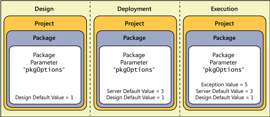
FIGURE 6-22 Parameter values by stage
